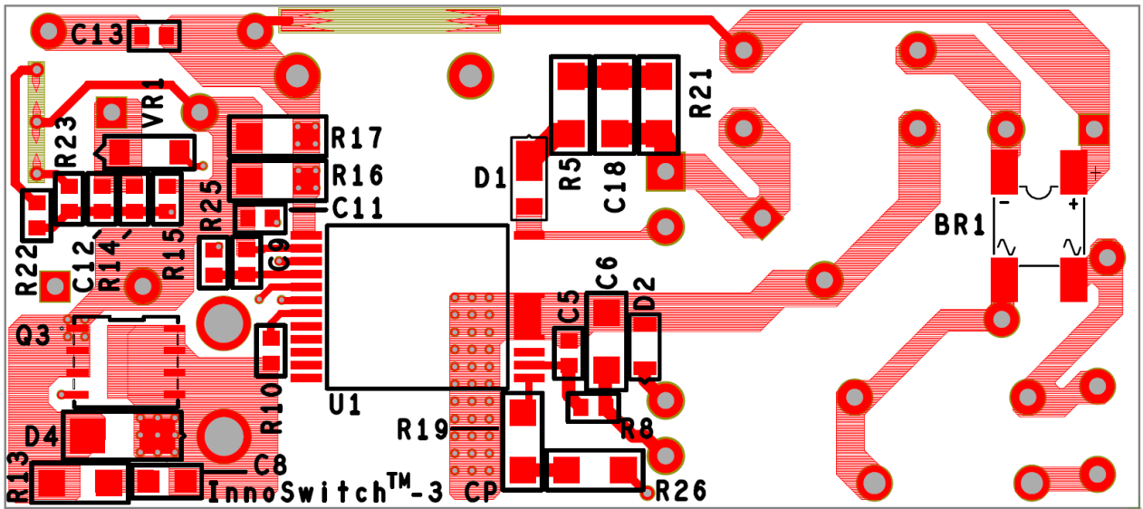
Figure 6 – Bottom Side.
