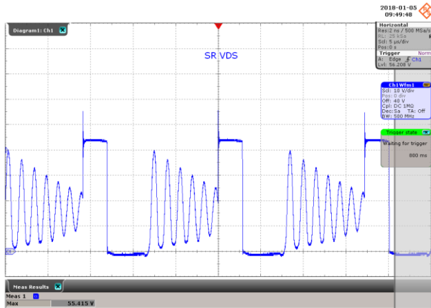
Figure 58 – SR FET Voltage Waveform. 180 VAC, 15.0 V, 2.0 A Load, (55.4 V MAX ). V DRAIN , 10 V, 5 µs / div.
