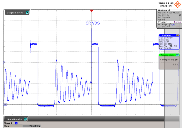
Figure 59 – SR FET Voltage Waveform. 265 VAC, 15.0 V, 2.0 A Load, (72.4 V MAX ). V DRAIN , 10 V, 5 µs / div.
