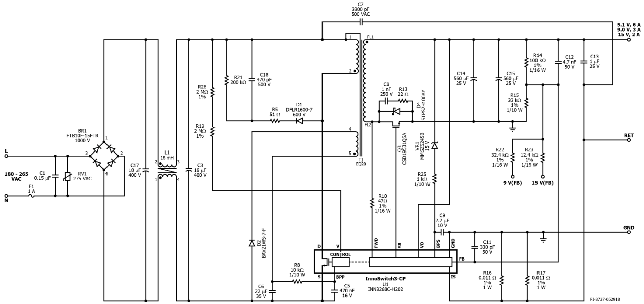
Figure 4 – Schematic.
