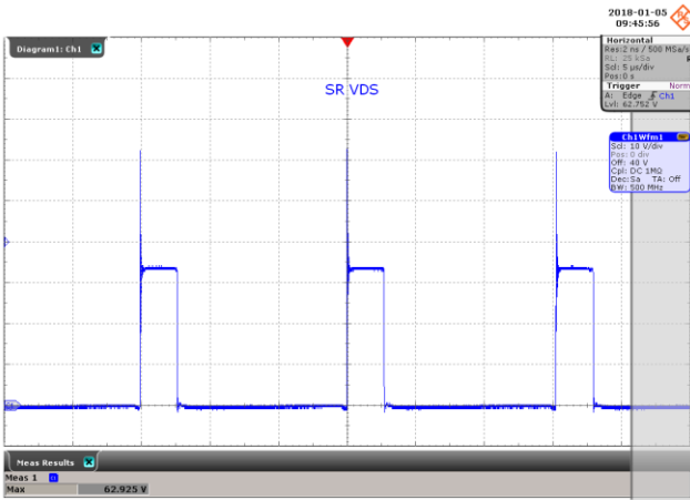
Figure 54 – SR FET Voltage Waveform. 180 VAC, 5.1 V, 6.0 A Load, (62.93 V MAX ). V DRAIN , 10 V, 5 μs / div.
