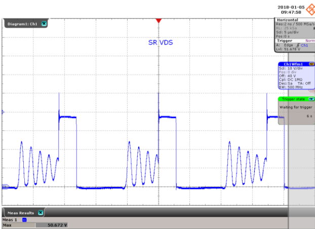
Figure 56 – SR FET Voltage Waveform. 180 VAC, 9.0 V, 3.3 A Load, (50.67 V MAX ). V DRAIN , 10 V, 5 μs / div.
